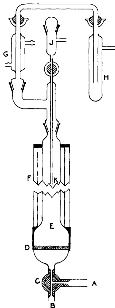
Fig. 1.—Oxidation apparatus.
