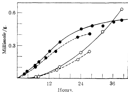
Fig. 2.—Autoxidation of diisopropyl ketone at 100°: ●, peroxide; ○, acid; light —, dark - - -.
