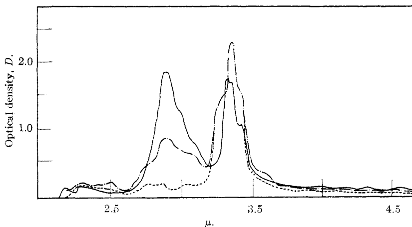
Fig. 4.—Infrared absorption spectra of diisopropyl ketone - - - (0.1), ketone oxidized at 110° for 32 hours — (0.1), and 2-(2,4-dimethylpentanone-3-yl) hydroperoxide — (0.05). Parenthetic numbers are cell thicknesses in mm.
