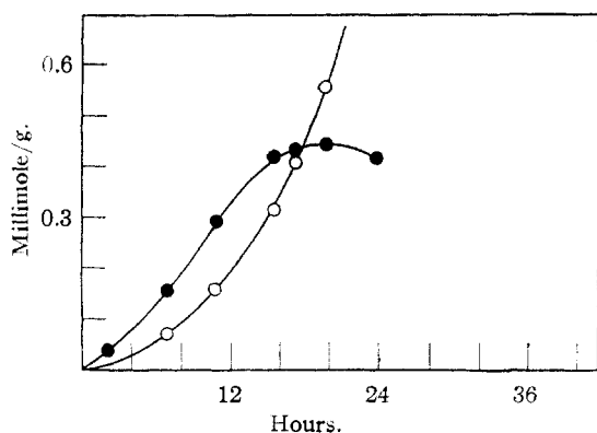
Fig. 3.—Autoxidation of diisopropyl ketone at 110°: ●, peroxide; ○, acid.
